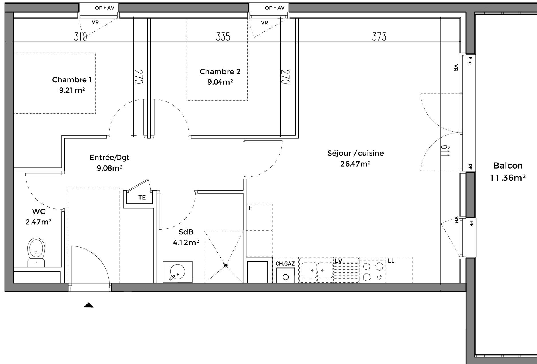
PLAN R+1
