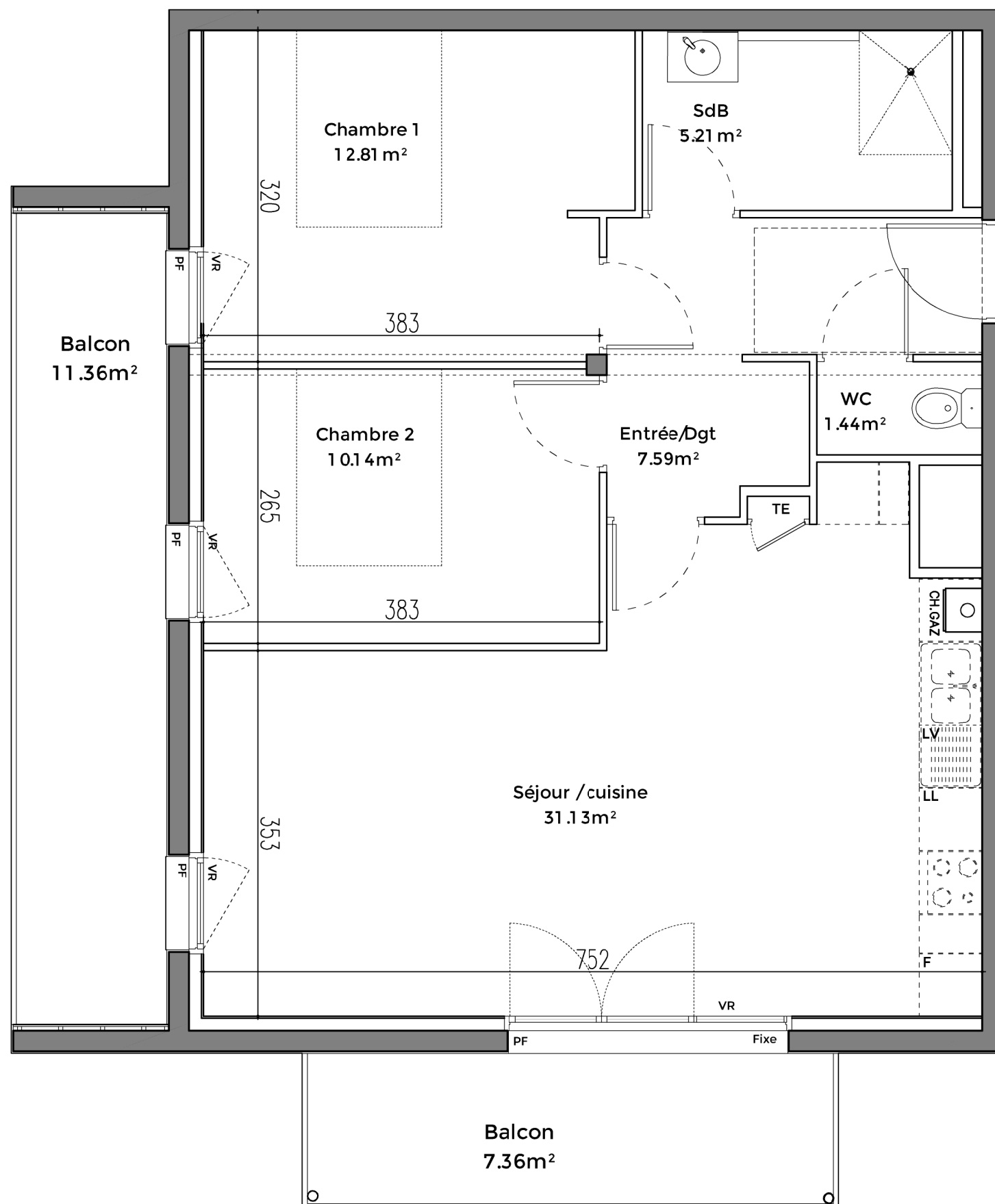
PLAN R+1
