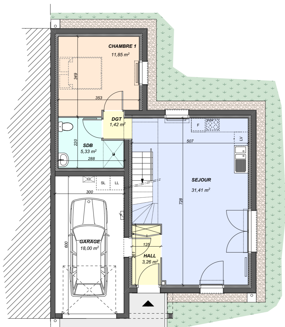
PLAN RDC 53,27m2
