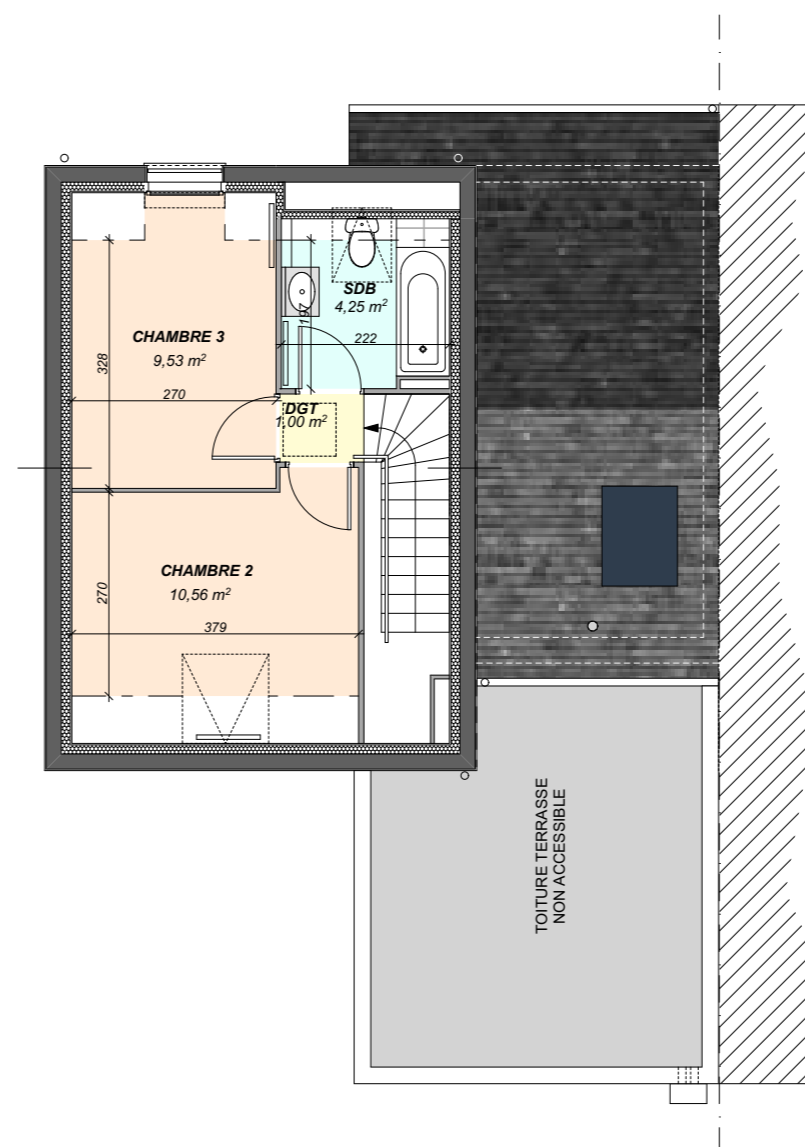
PLAN R+1 25,34m 2
