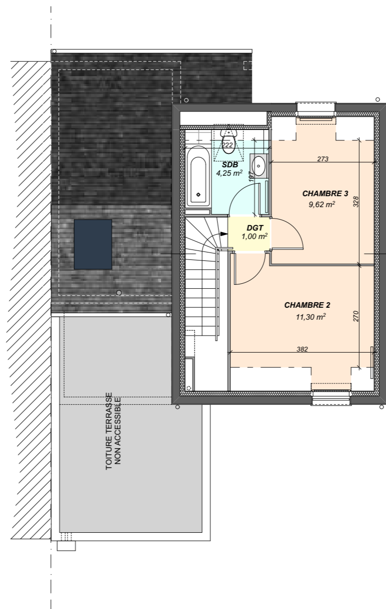
PLAN R+1 26,17m2
