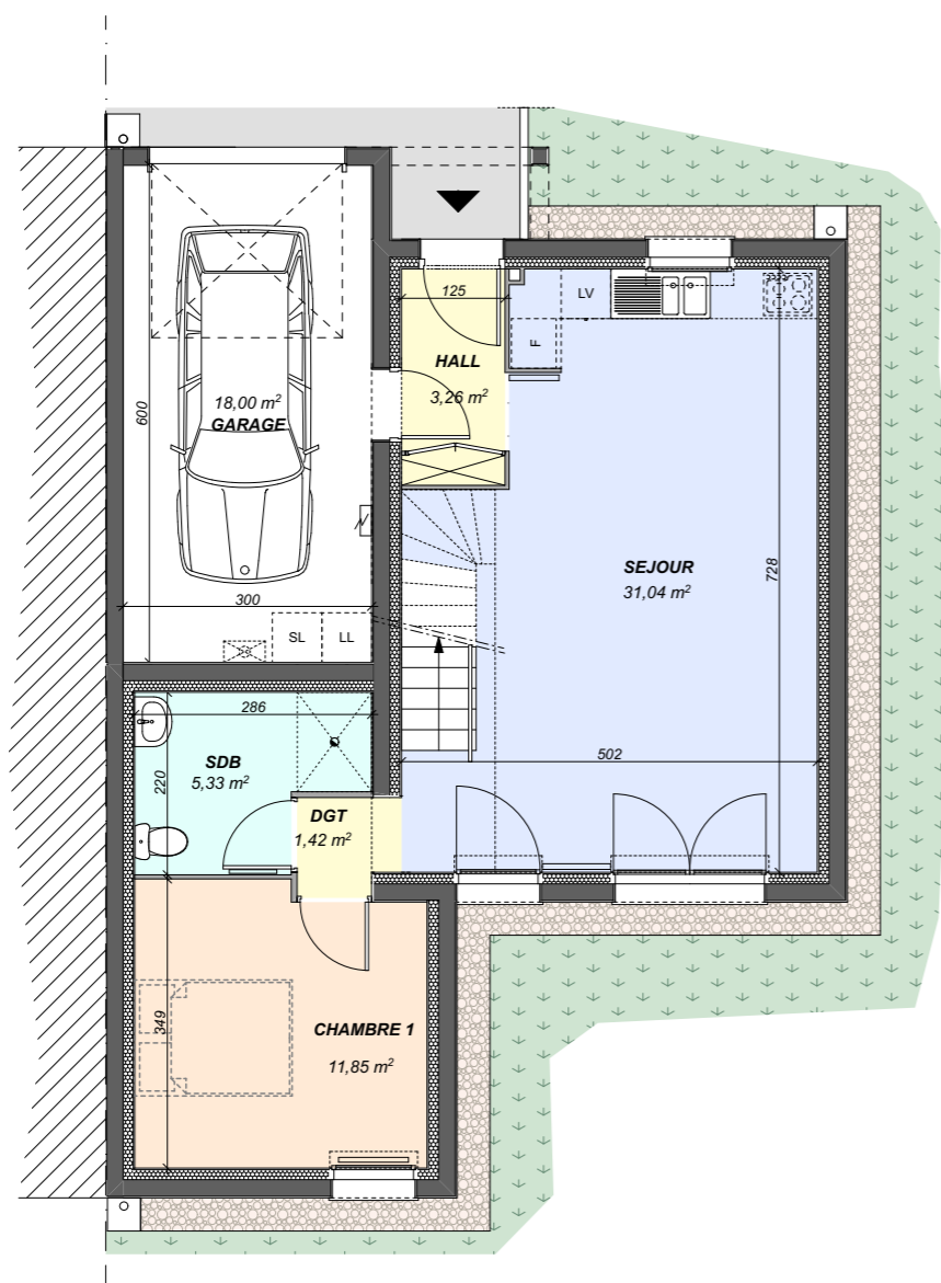
PLAN RDC 52,90m2
