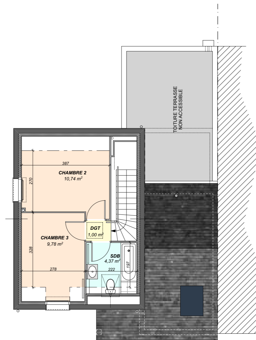
PLAN R+1 25,89m2
