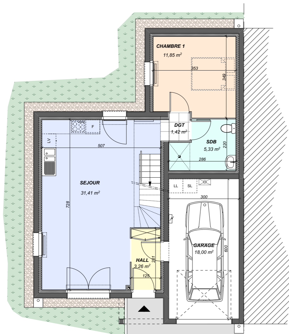
PLAN RDC 53,27m2
