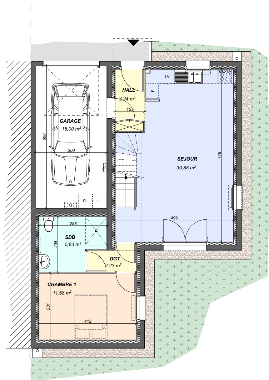
PLAN RDC 53,76m 2
