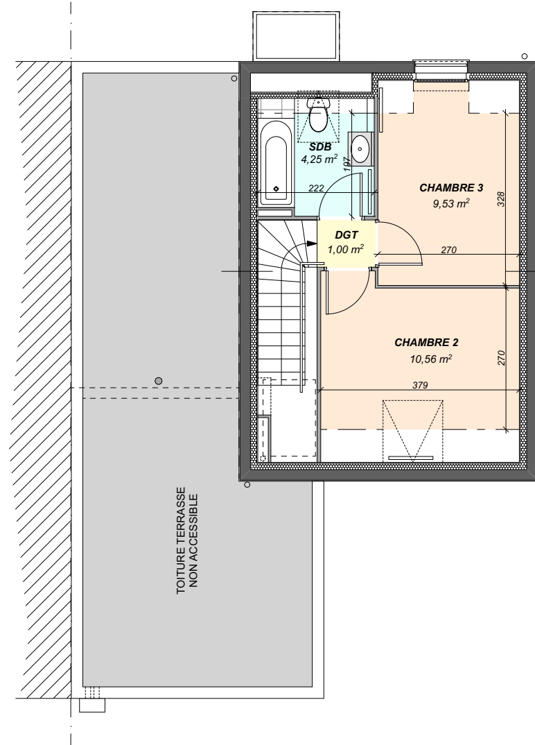
PLAN R+1 25,34m 2
