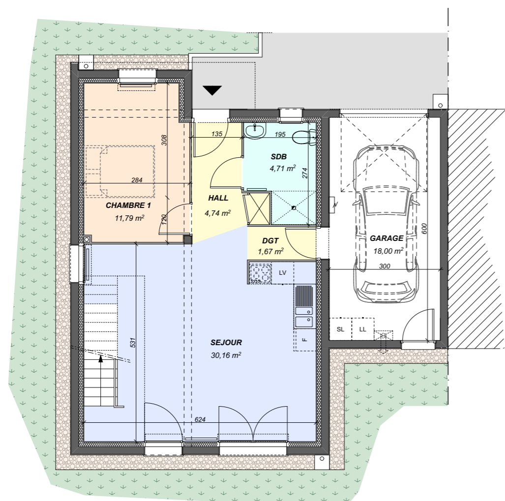
PLAN RDC 53,07m2
