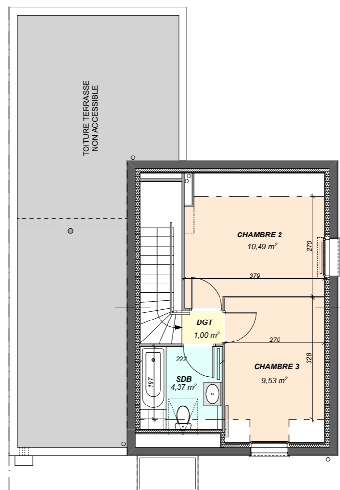
PLAN R+1 25,39m2
