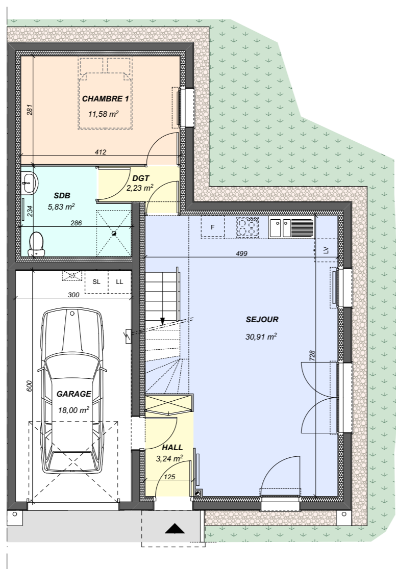
PLAN RDC 53,79m2
