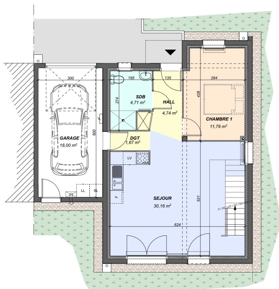
PLAN RDC 53,07m 2
