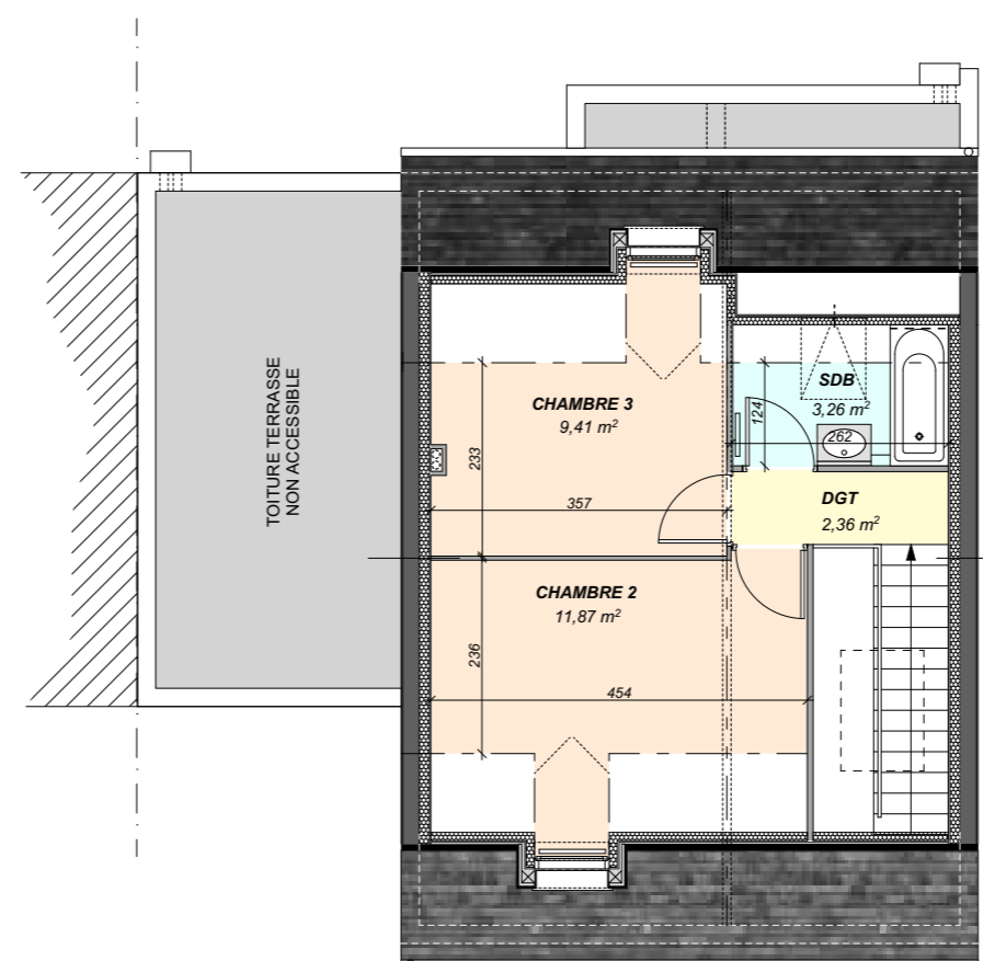
PLAN R+1 26,90m 2
