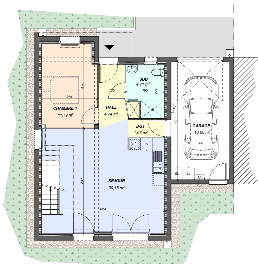
PLAN RDC 53,07m2
